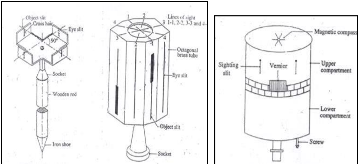
Figure :Cross staff
