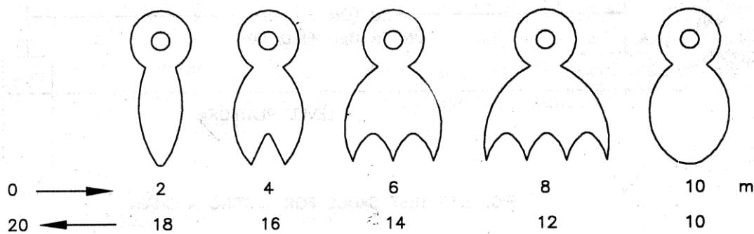
FIG. 2.12 TALLIES FOR A 20 METRE CHAIN
